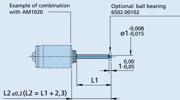
Version with bearing tip M1,6 x 0,35 x L1 T
